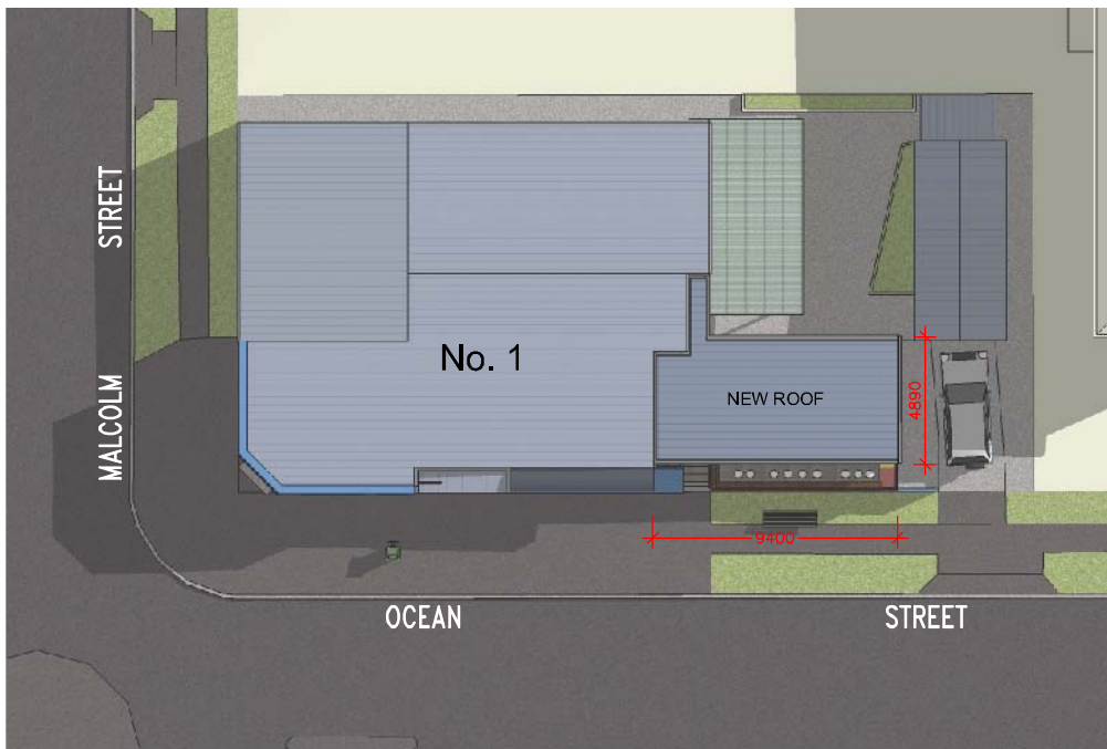
SITE PLAN
